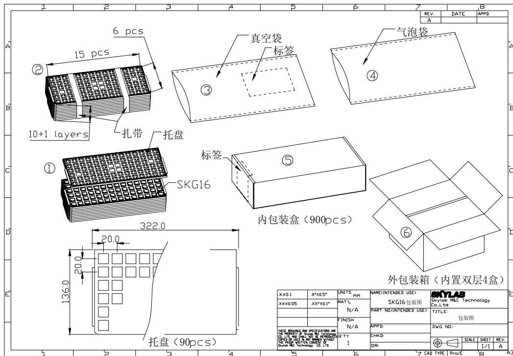
Figure 4: SKG16 Series Packaging
