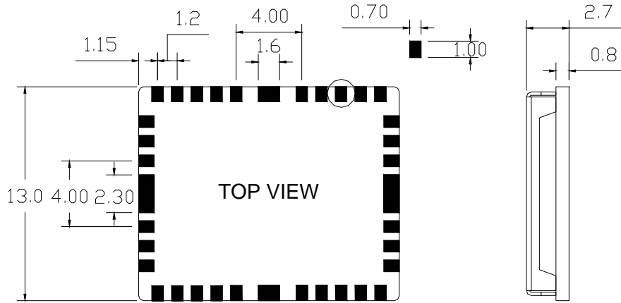
Figure 3: SKG16 Series Dimensions
