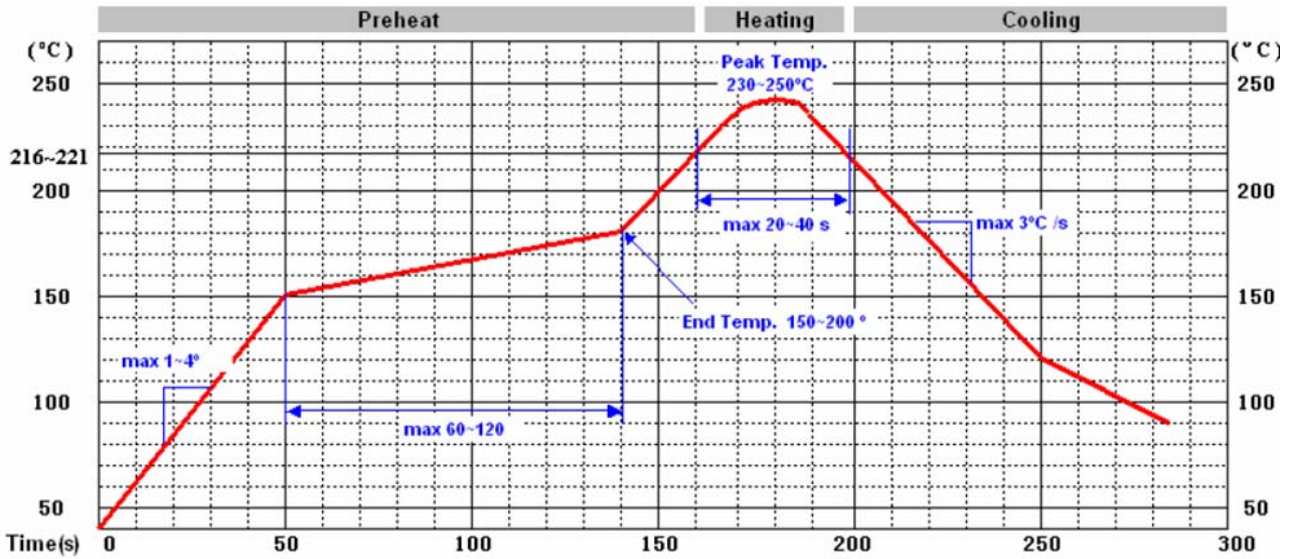
Figure 5: SKG16 Series Typical Leadfree Soldering Profile
