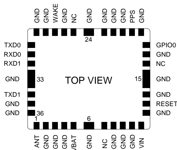
Figure 2: SKG16 Series Pin Package
