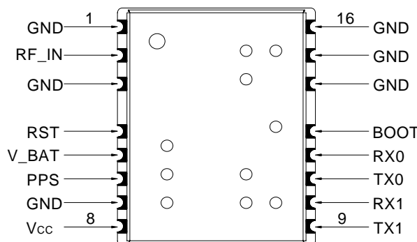
Figure 2: GM20 Pin Package
