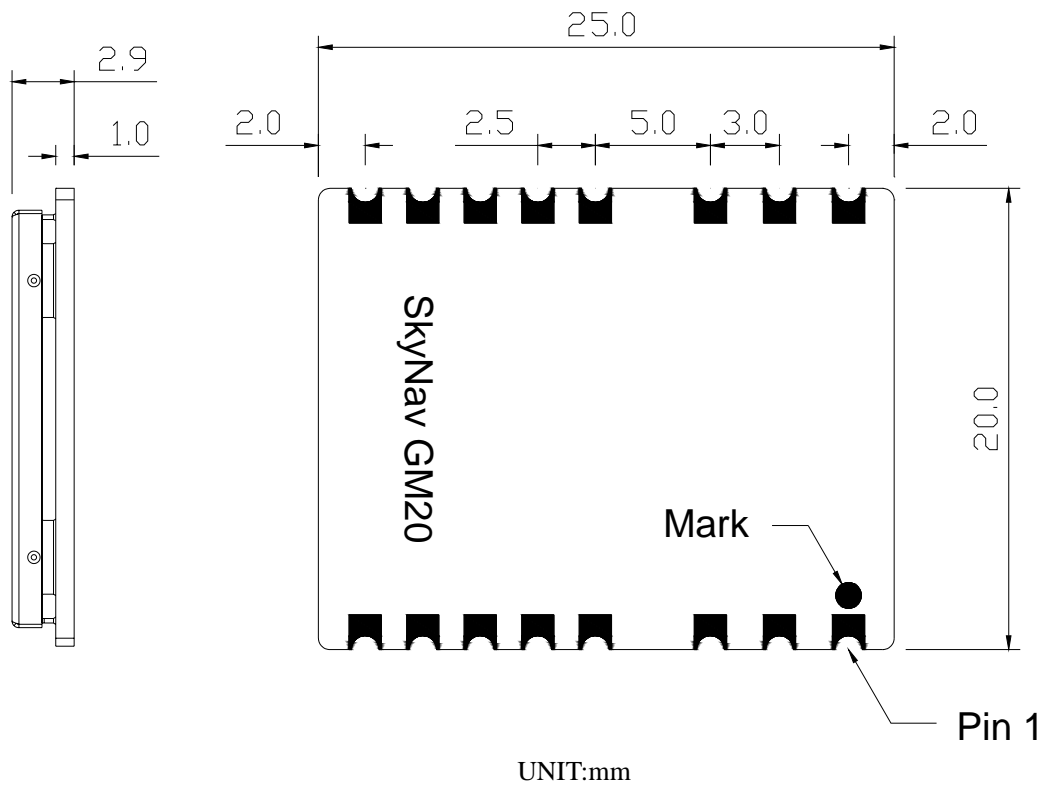
Figure 3: GM20 Dimensions
