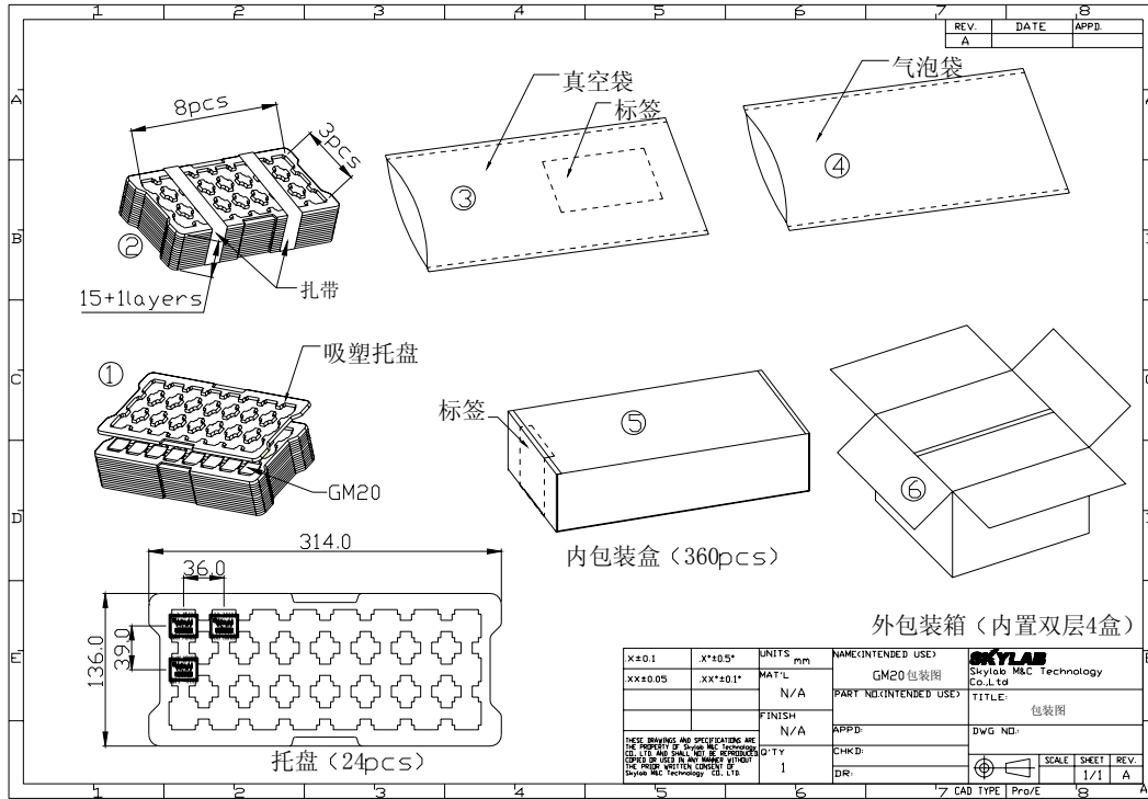
Figure 4: GM20 Packaging
