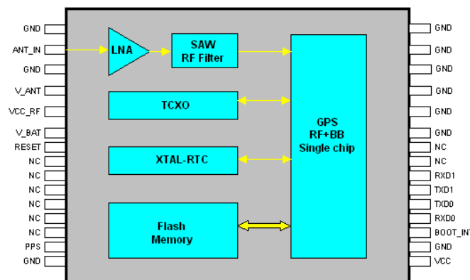
Figure 2: GM25 Pin Package
