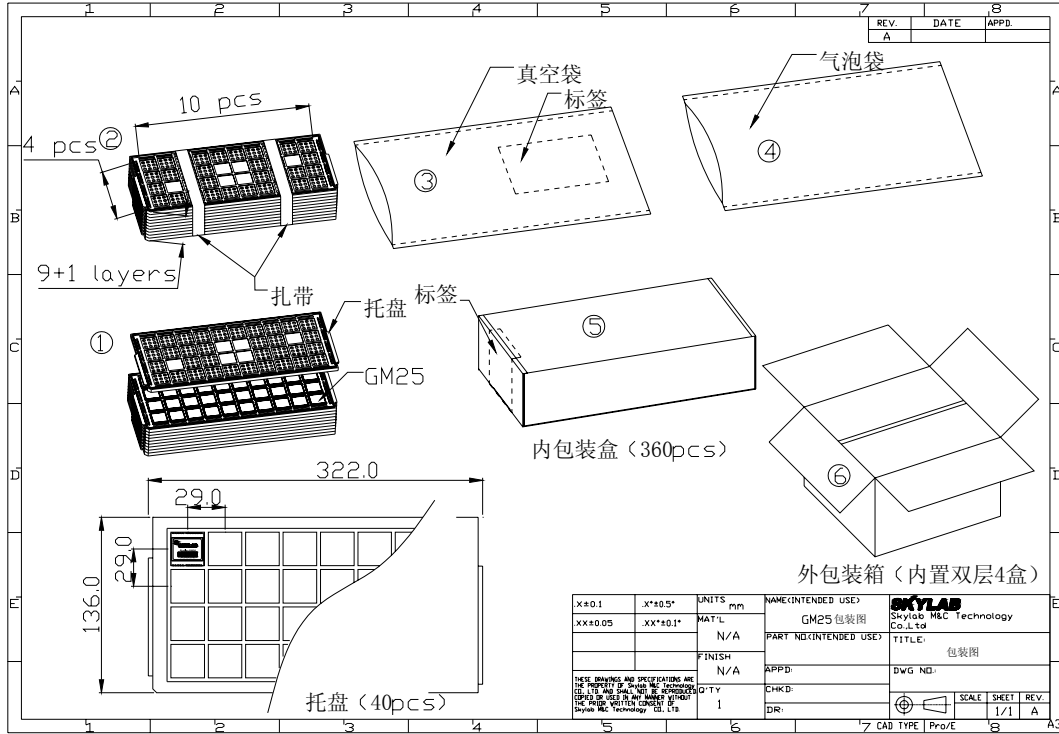
Figure 4: GM25 Packaging
