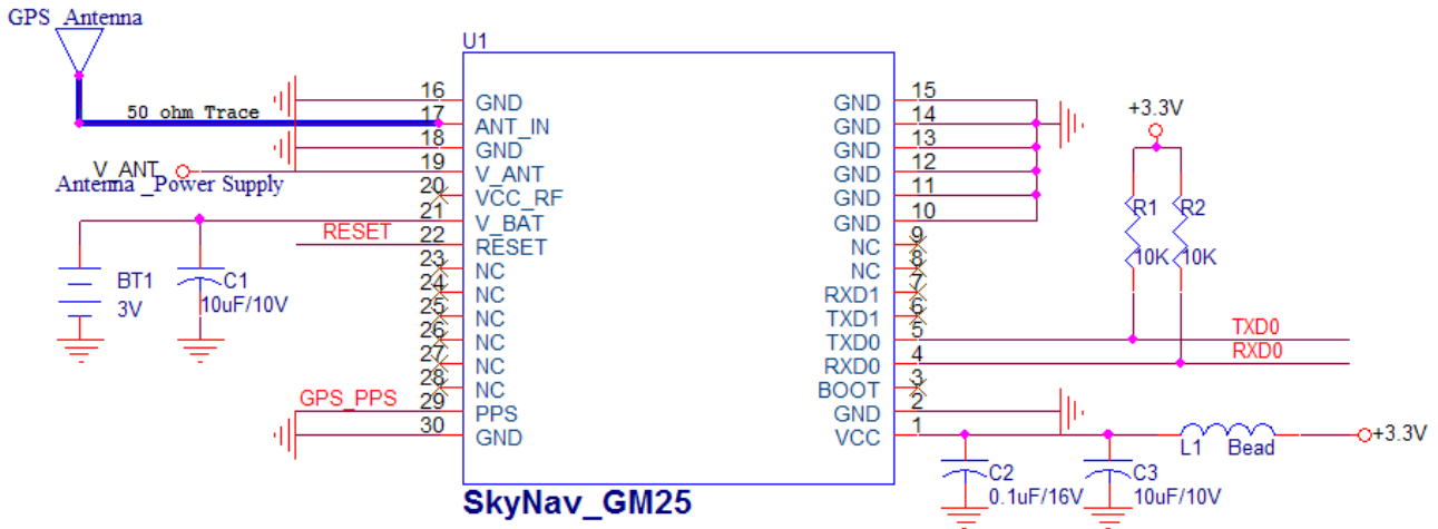
Figure 6: GM25 Typical Reference design schematic
