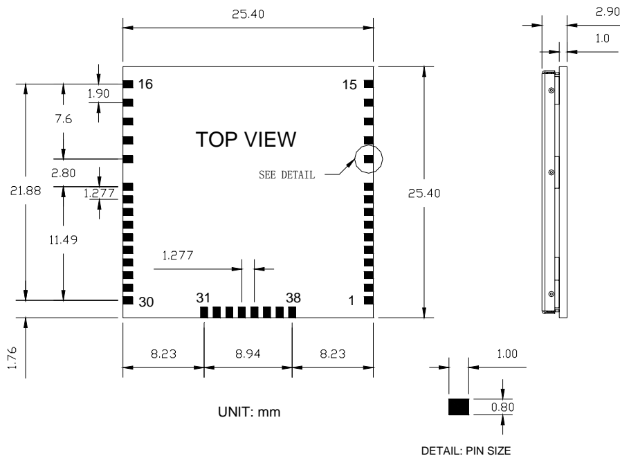
Figure 3: GM25 Dimensions
