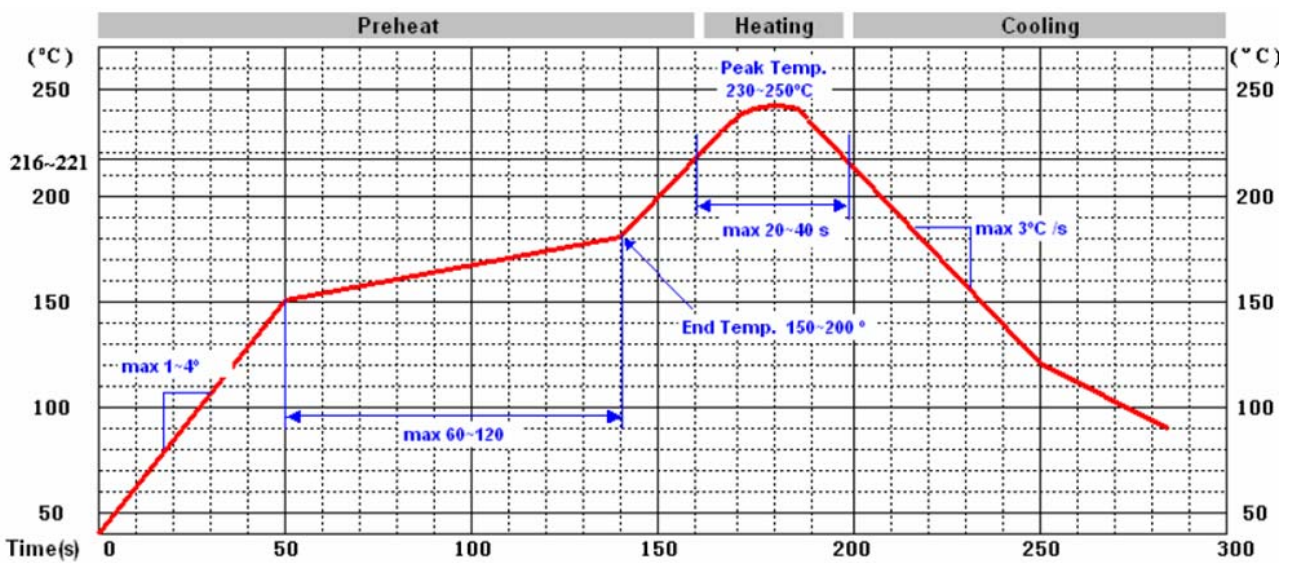
Figure 5: GM25 Typical Leadfree Soldering Profile
